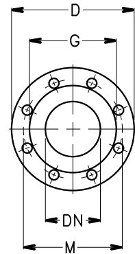
PUMP FLANGES
