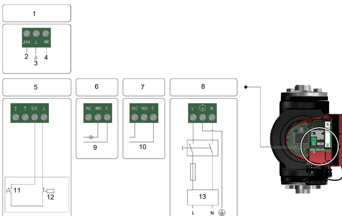
Example of connections in the control box of a terminal-connected version
