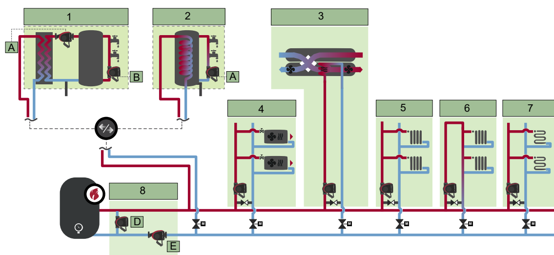
Functional drawing of a heating system in a commercial building
