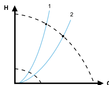
Hydraulic difference between the pump head to the right (1) and to the left (2) of the flap valve
