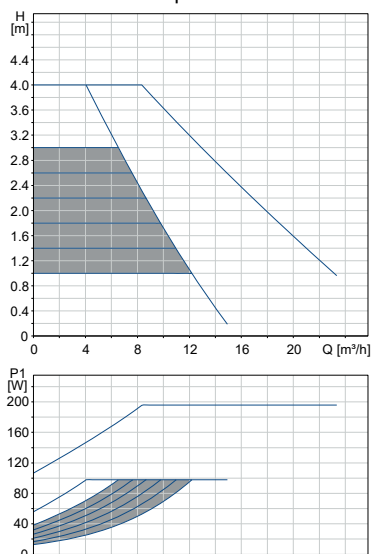
Constant pressure
