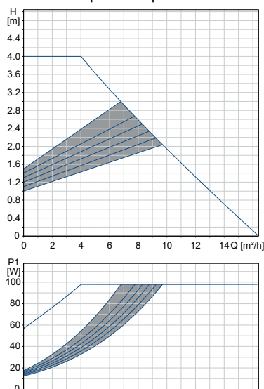
Proportional pressure
