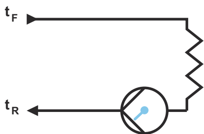
Fig. 24 Pump with internal sensor
