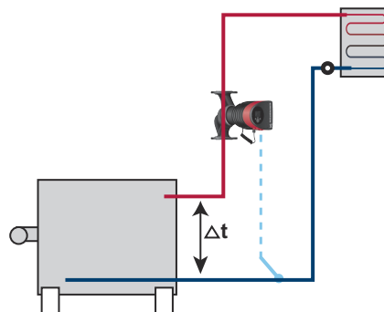
Fig. 21 Differential temperature
