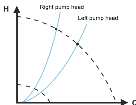
Fig. 33 Hydraulic difference between the two heads
