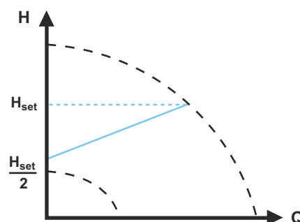
Fig. 17 Proportional-pressure control
