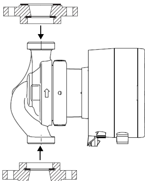
Fig. 73 Example of thread-flange adapters
