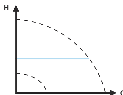
Fig. 18 Constant-pressure control
