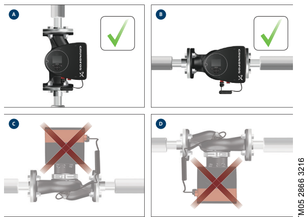
Fig. 49 Installation positions
