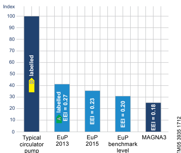
Fig. 60 Energy consumption index
