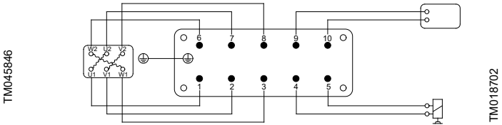
Plug connection from the motor
