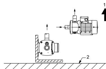
Positions of the CM self-priming pumps
