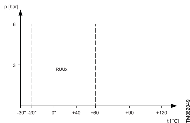
Curve for the RUUx shaft seal
