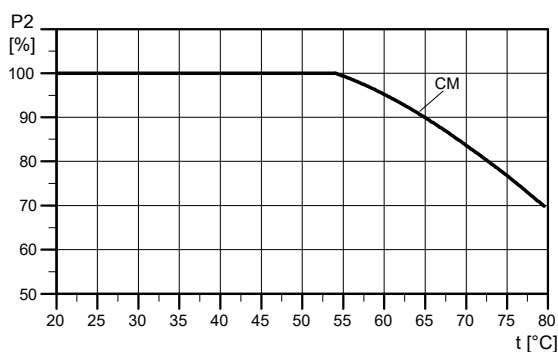
Derating of the CM pump in relation to ambient temperature
