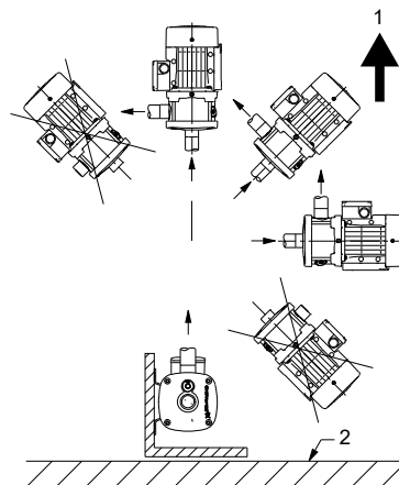
Positions of the CME and CM pumps
