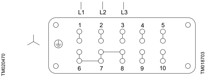
Plug connection for star connection
