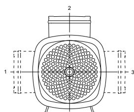
Terminal box positions of frame sizes 71 and 80, as seen from the fan cover side
