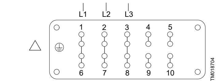
Plug connection for delta connection
