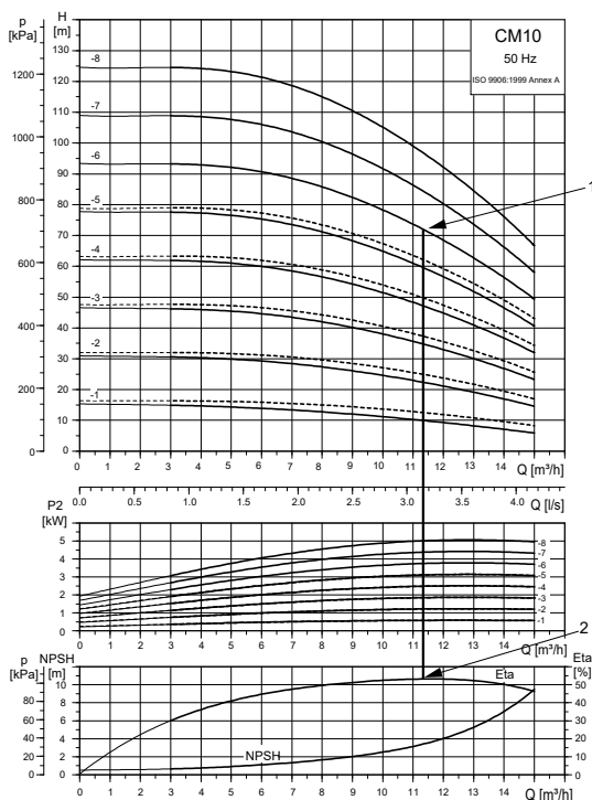
Example of the duty point of a CM pump
